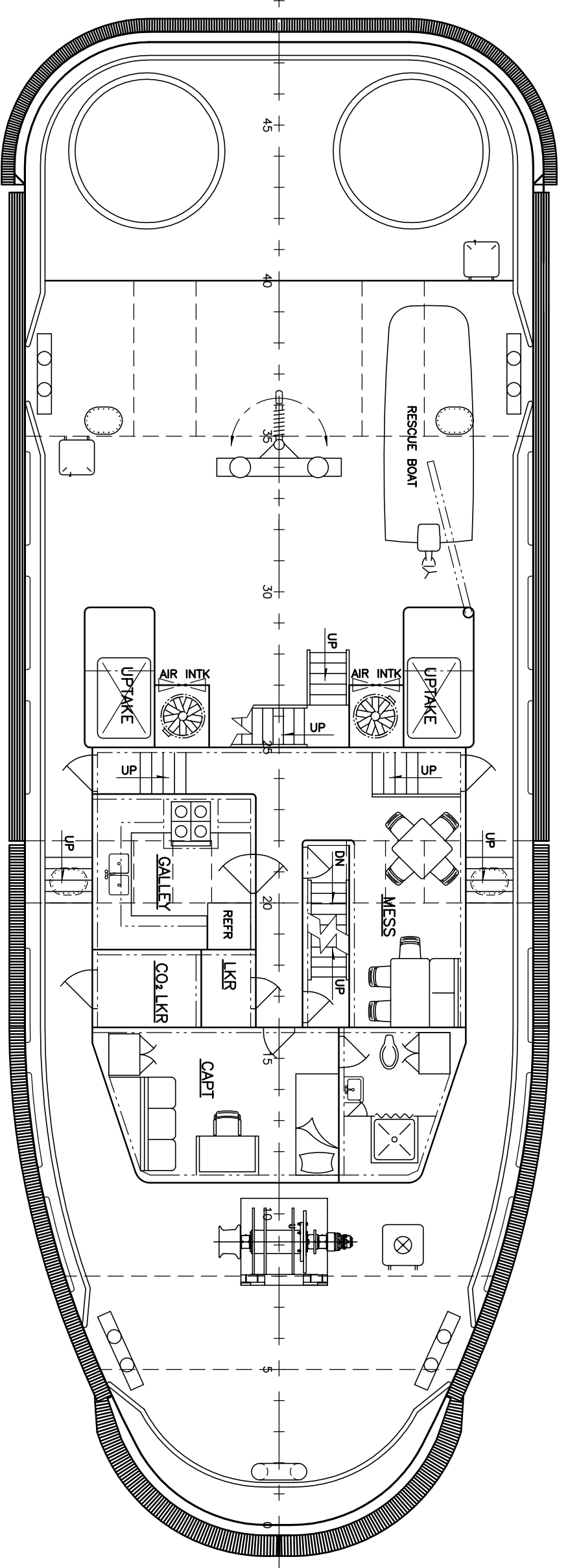
MAIN DECK PLAN
